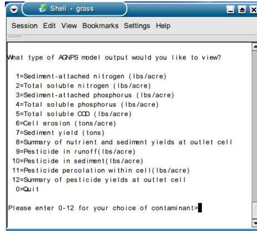
Figure 9: shows menu interface of r.agnps50.view
