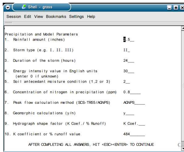
Figure 3: Precipitation parameters
