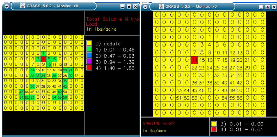
Figure 10: shows Total soluble nitrogen and Pesticide in runoff
