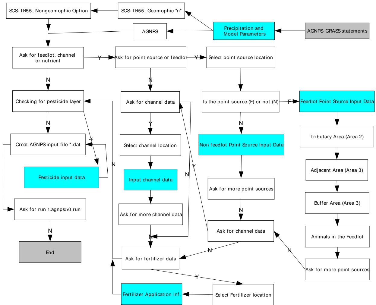
Figure 8: Flow of input interface of r.agnps50.input
